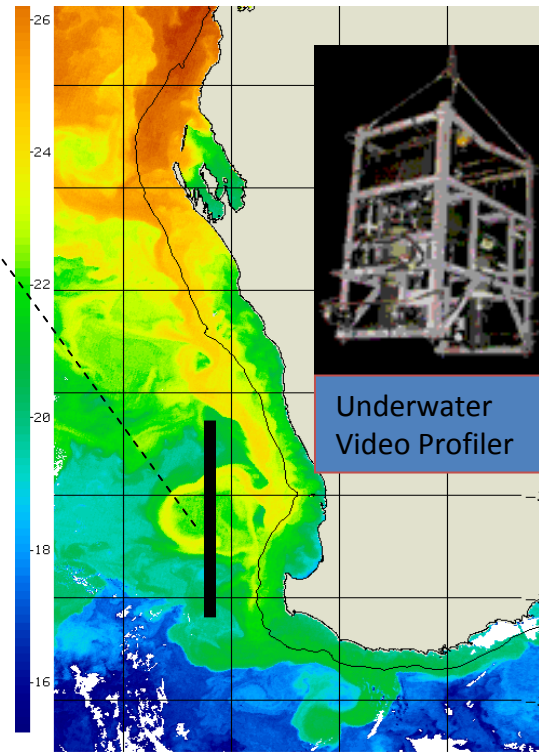
NOAA17 SST 11 May 2006 0227Z Copyright 2006, CSIRO Marine Research, Hobart
